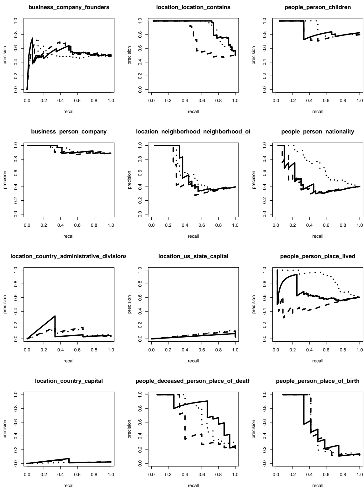
Figure 5.6: Per-relation precision and recall on the sentence-level relation extraction task. The dashed line corresponds to MultiR, DNMR is the solid line, and DNMR*, which incorporates side-information, is represented by the dotted line.
