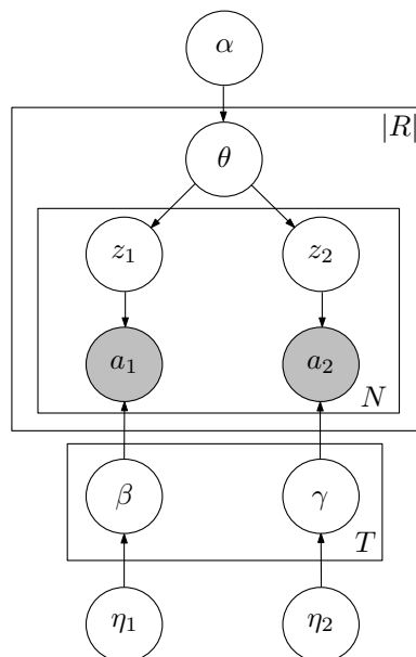
Figure 6.2: LinkLDA
