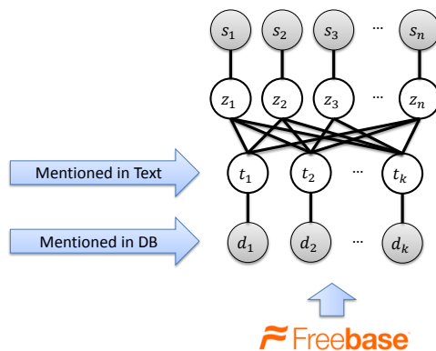
Figure 5.3: DNMAR
