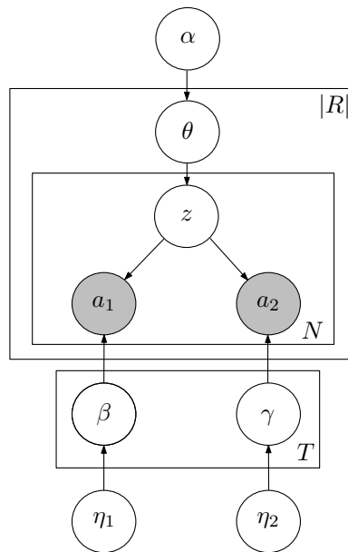
Figure 6.1: JointLDA
